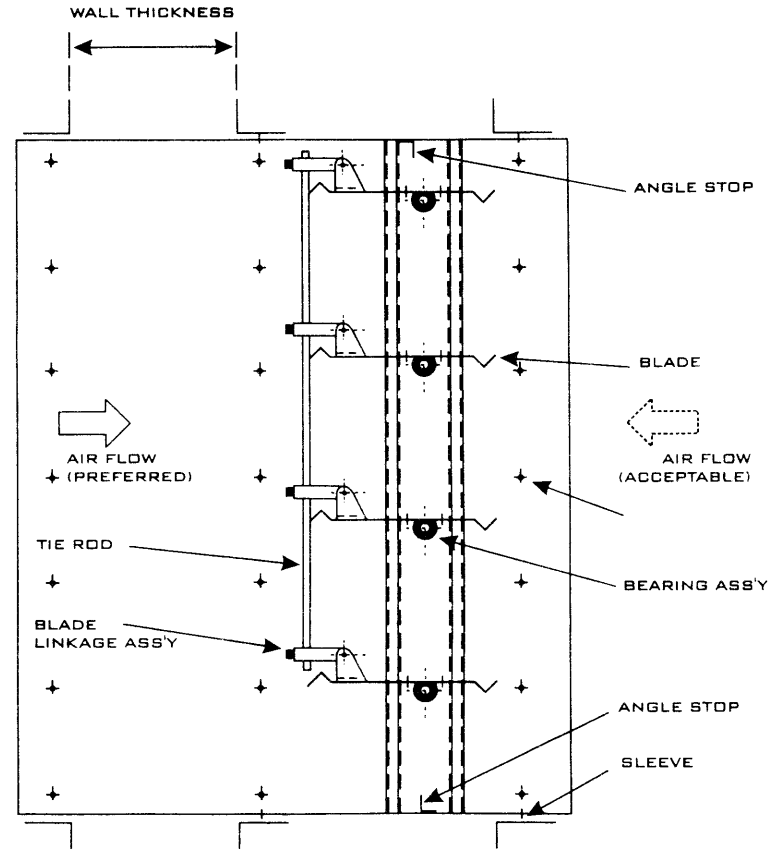
SECTION THRU OPEN POSITION
